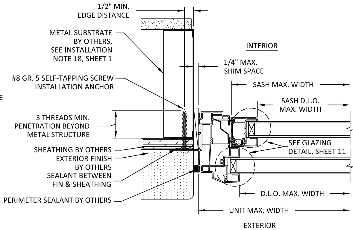
B 7 HORIZONTAL SECTION NAIL FIN INSTALLATION METAL STUD
