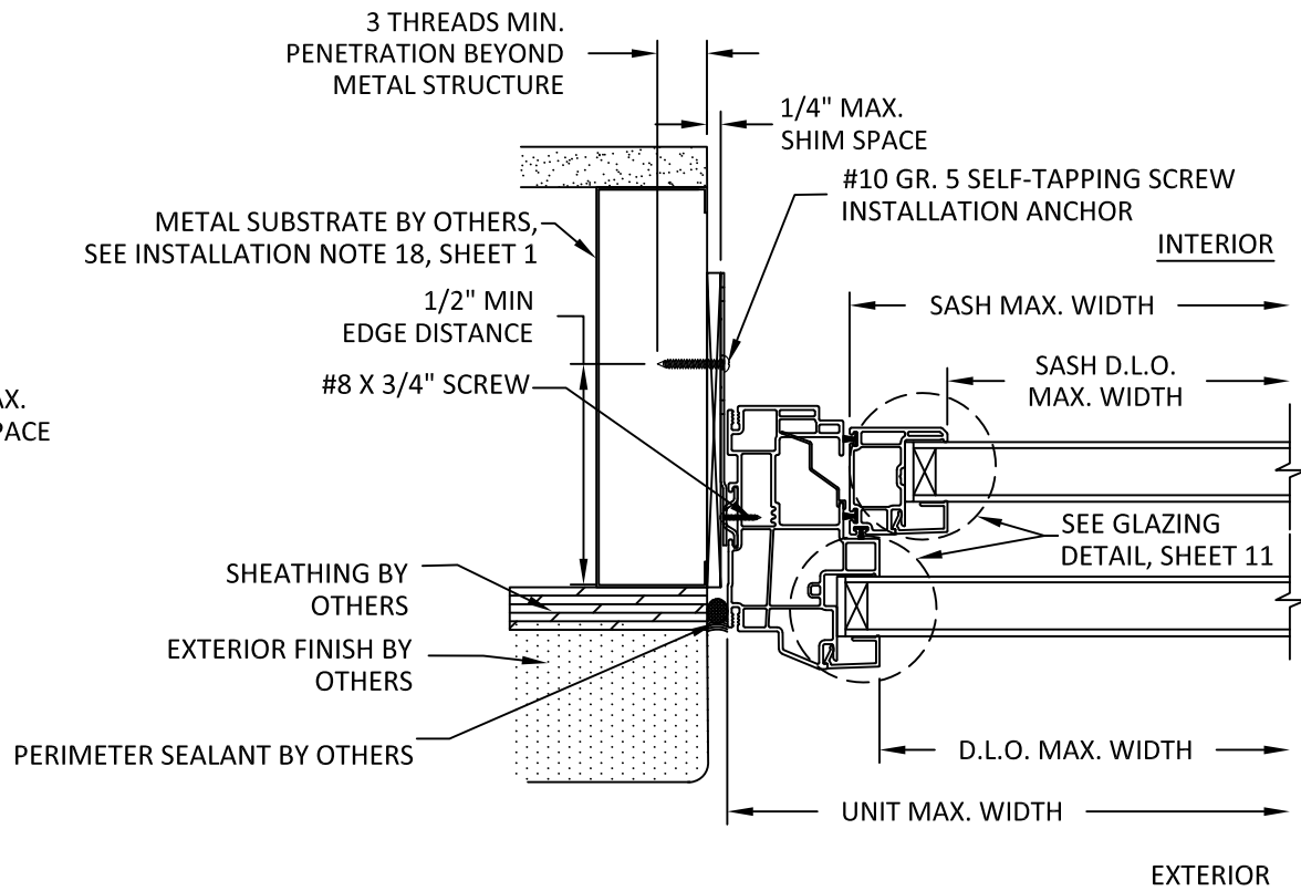
B 9 HORIZONTAL SECTION CLIP INSTALLATION METAL STUD
