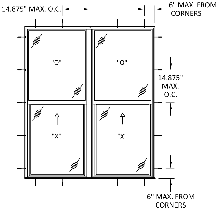
ANCHOR LAYOUT CLIP INSTALLATION
