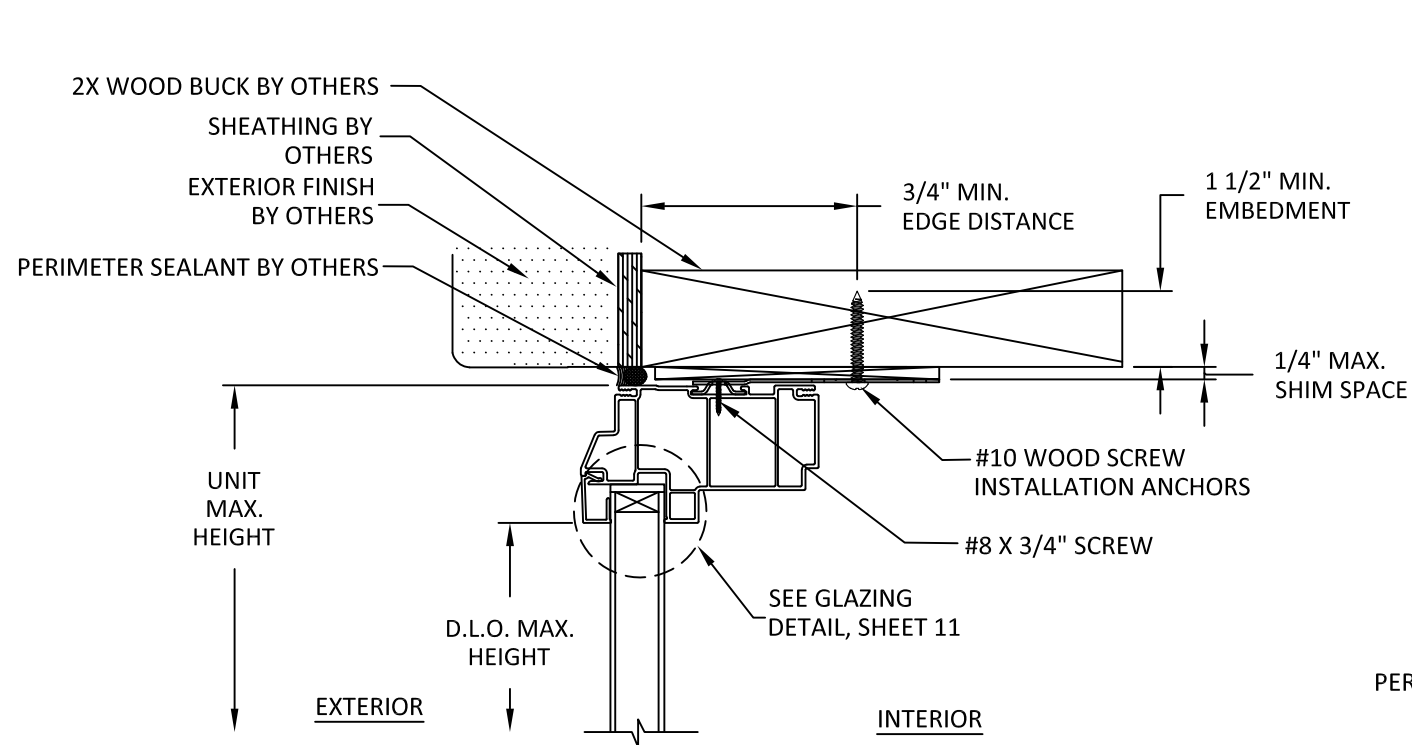
A 9 VERTICAL SECTION CLIP INSTALLATION WOOD BUCK
