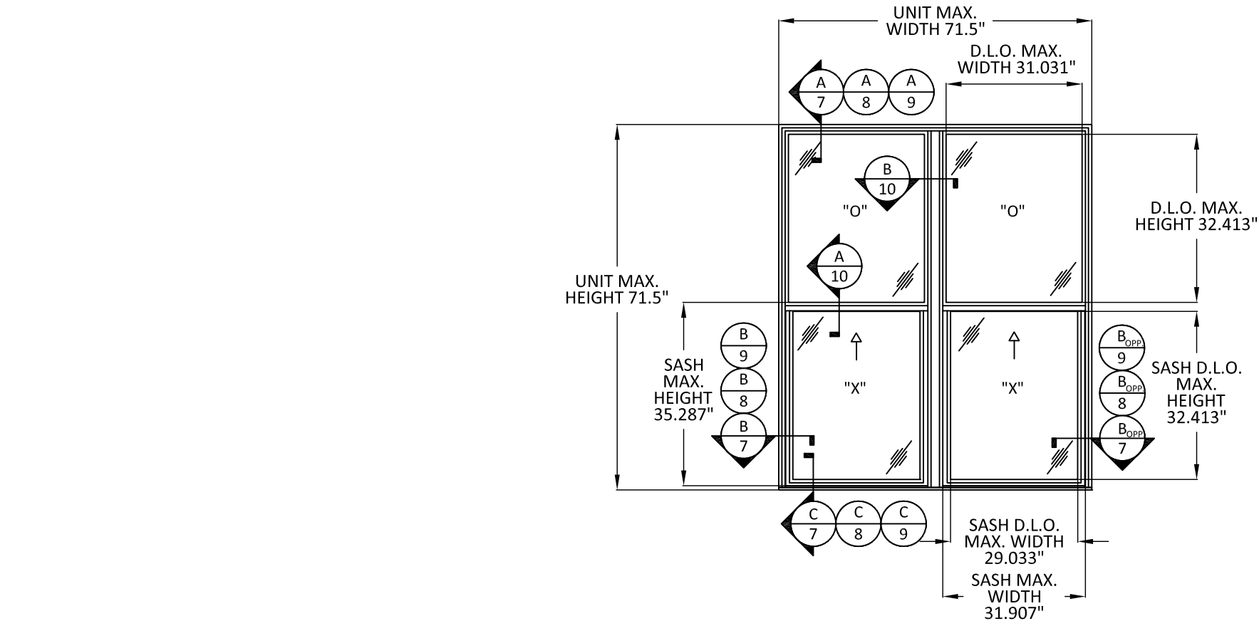
TYPICAL ELEVATION SINGLE HUNG TWIN
