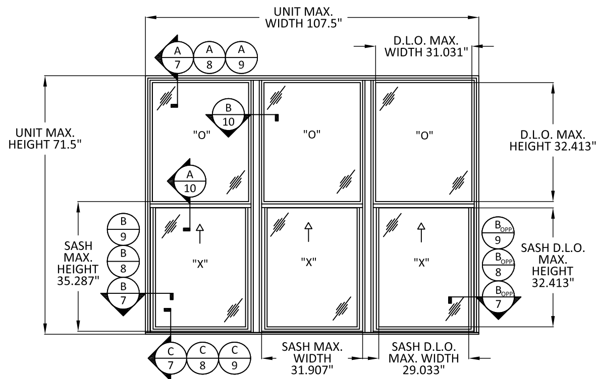
TYPICAL ELEVATION SINGLE HUNG TRIPLE
