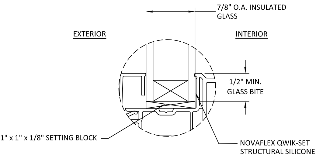
GLAZING DETAIL
