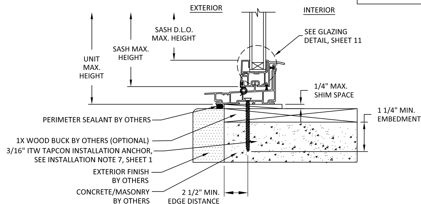
C 8 VERTICAL SECTION THROUGH FRAME INSTALLATION CONCRETE/CMU
